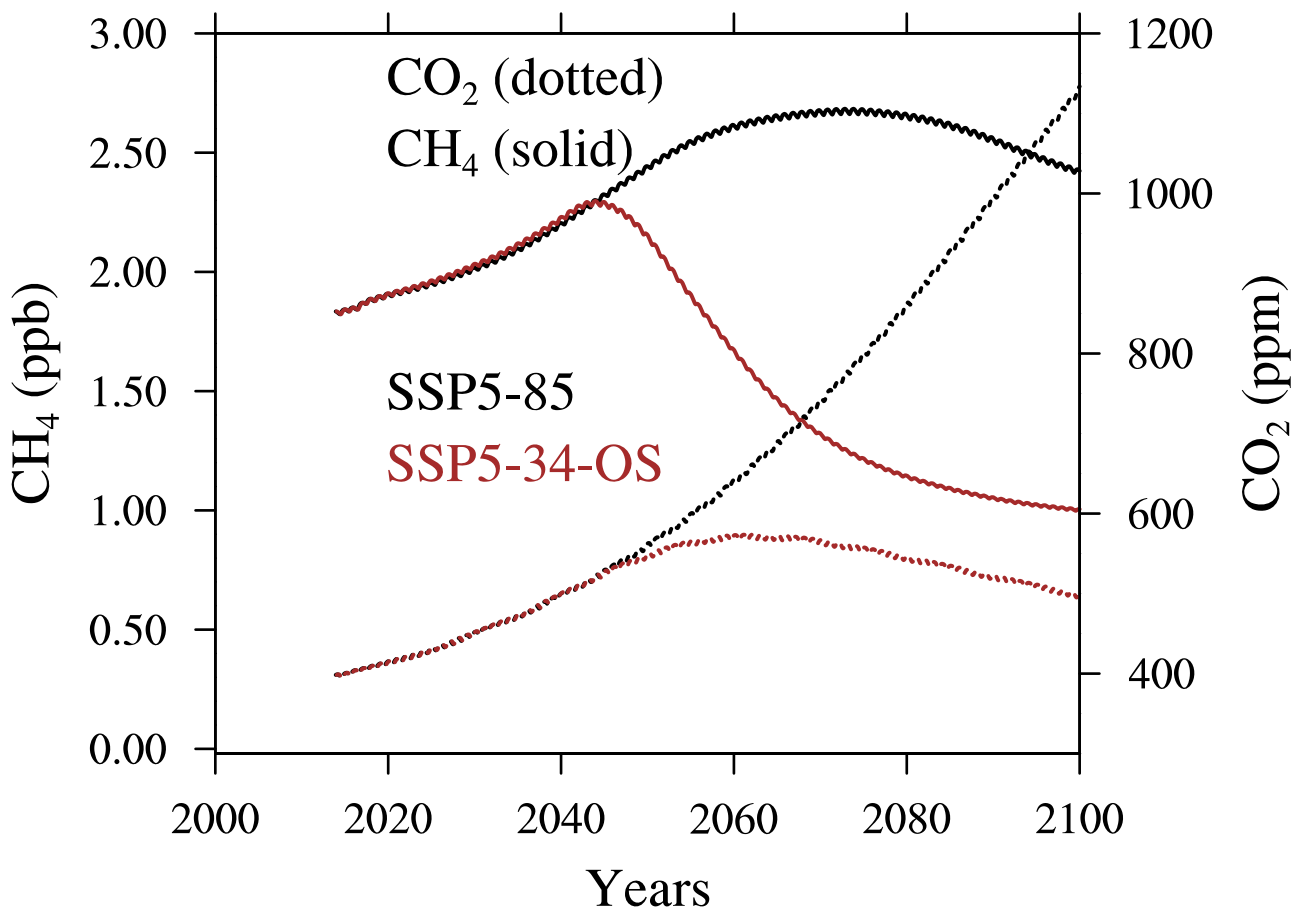
(b) Lower boundary conditions
