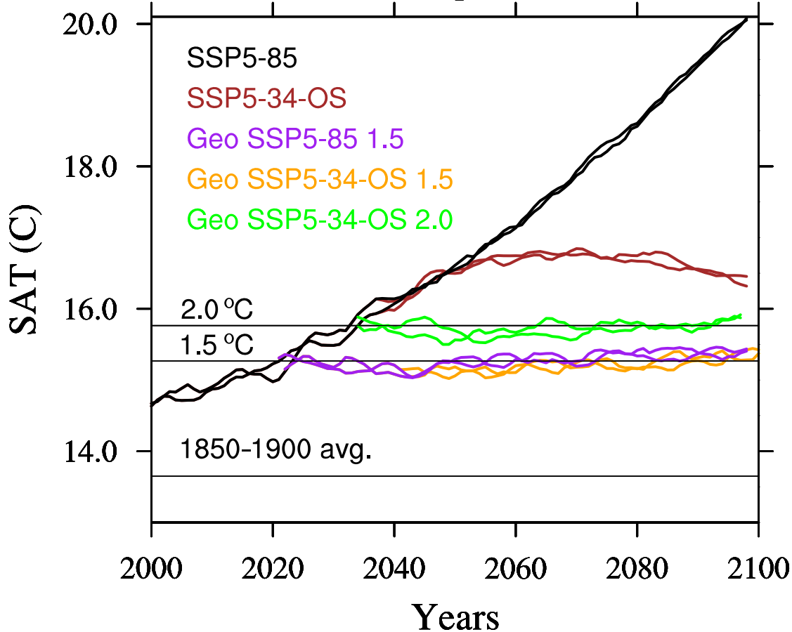
(a) Surface air temperature ( ^{\circ}\text{C} )
