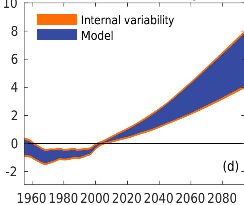
Sources of uncertainty (%)
