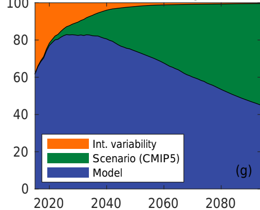
Fractional contribution to total uncertainty (%)
