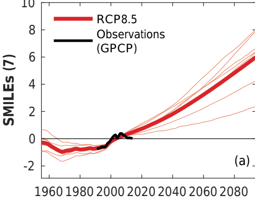
Global decadal mean annual precipitation (%) relative to 1995–2014
