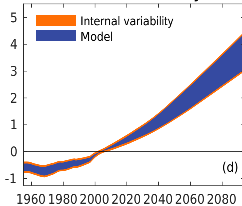
Sources of uncertainty (K)
