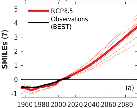
Global decadal mean annual temperature (K) relative to 1995–2014
