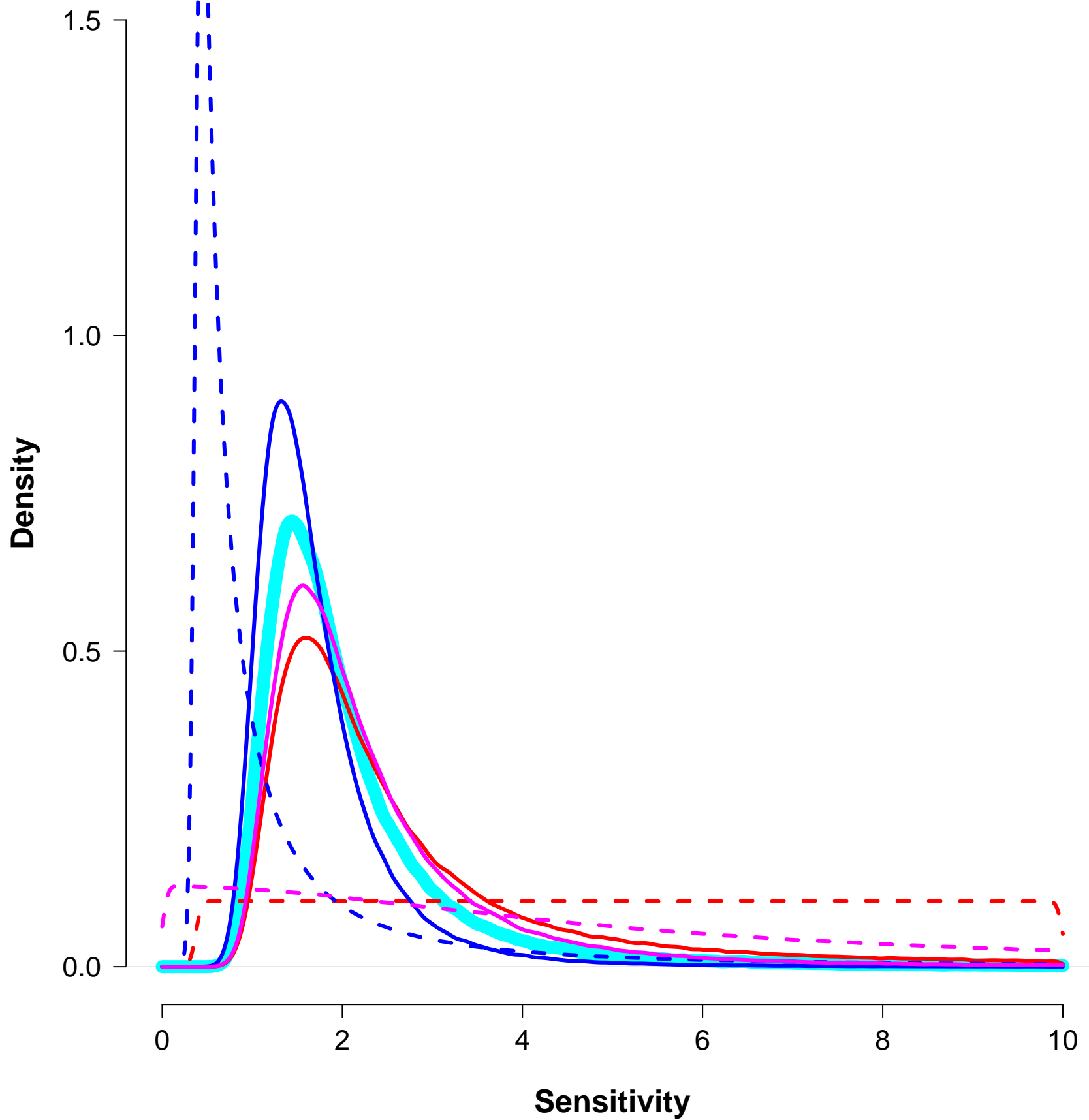
Priors and posteriors for Bayesian estimate using 20th century data
