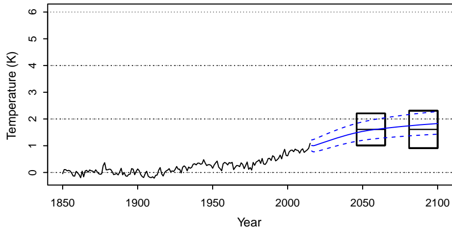
(c) RCP6 (scaling)
