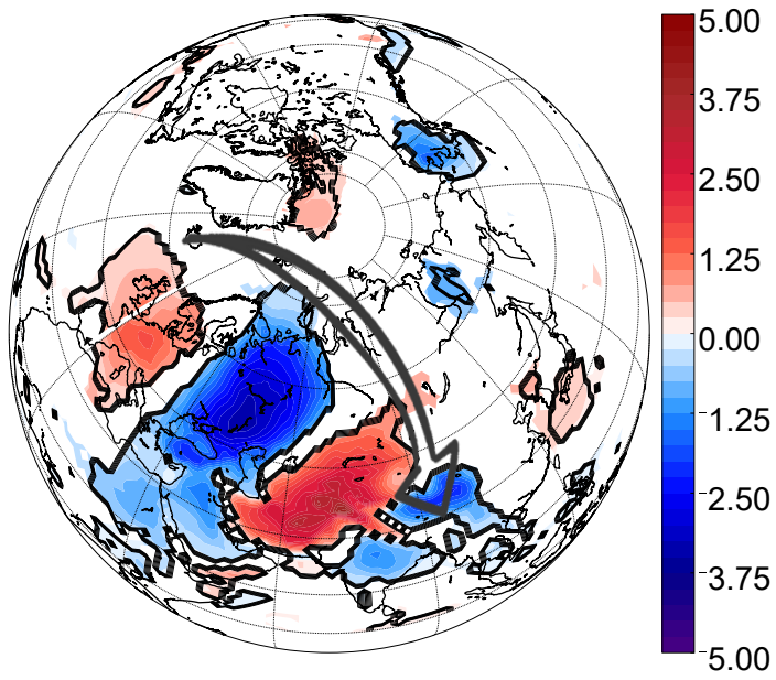
(e) T anomalies associated with CGTI (K)
