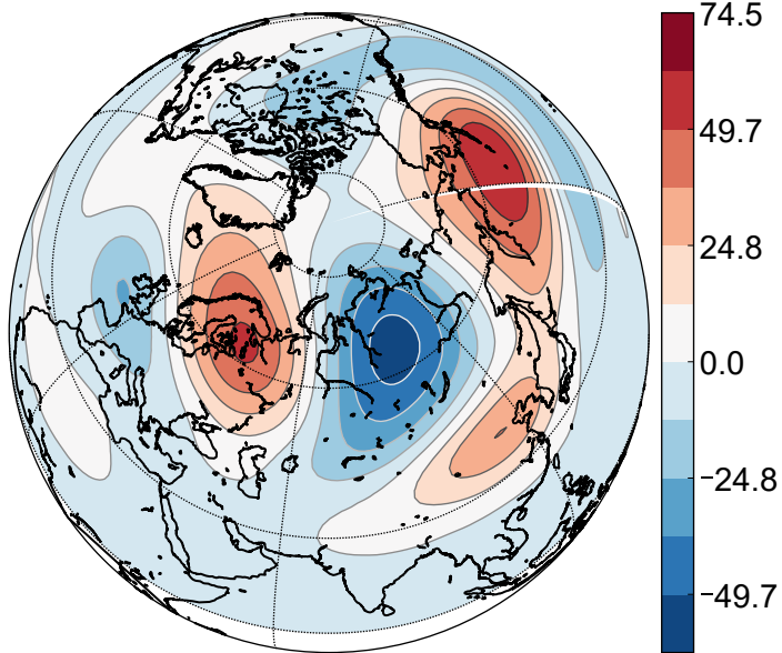
(a) EOF1 of weekly Z200 (JJAS)
