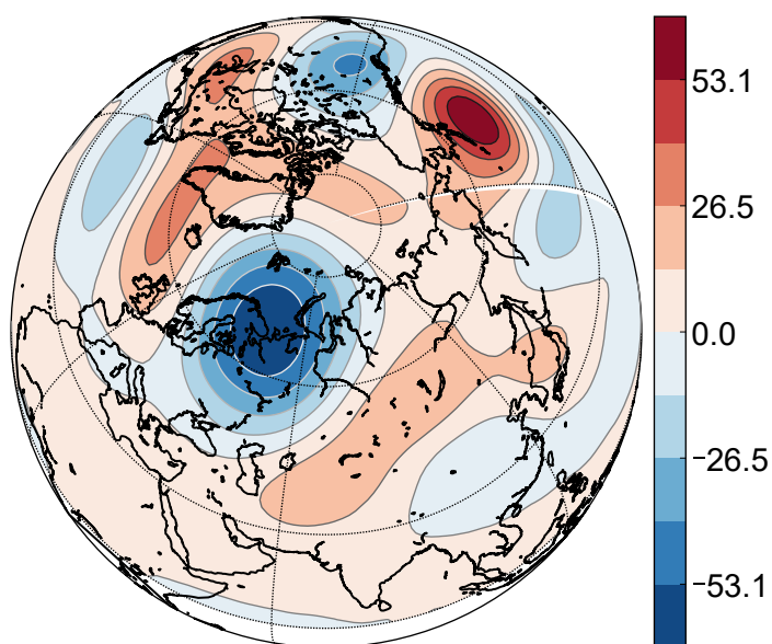
(b) EOF2 of weekly Z200 (JJAS)
