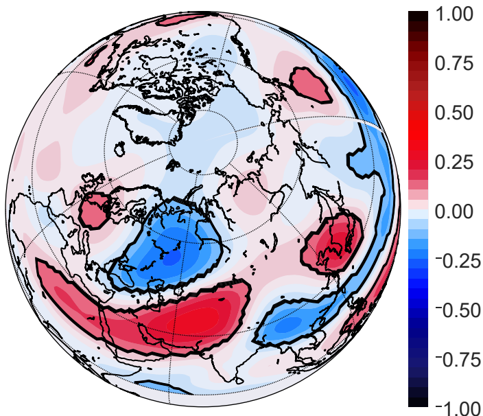
(c) Lag -1 correlation of Z200 with MT rain
