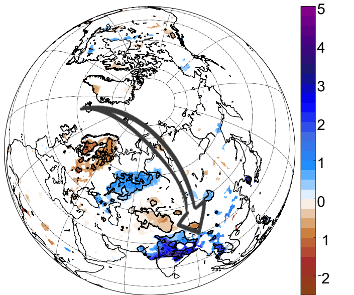
(f) P anomalies associated with CGTI ( \text{mm d}^{-1} )
