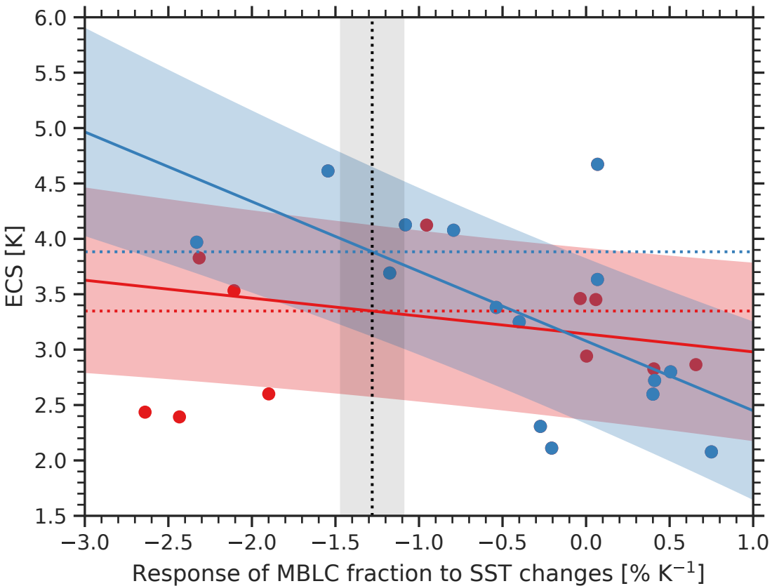
Zhai et al. (2015) constraint (ZHA) for CMIP5
