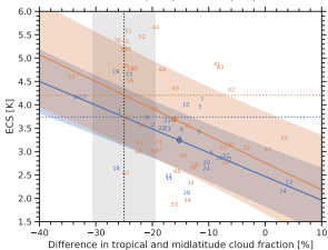
Volodin (2008) constraint (VOL)
