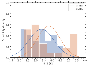
Zhai et al. (2015) constraint (ZHA)
