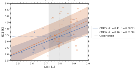
Sherwood et al. (2014) constraint (SHS)
