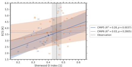
Sherwood et al. (2014) constraint (SHL)
