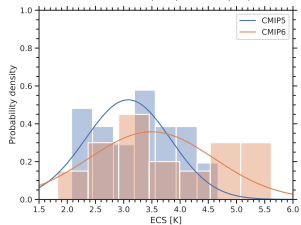
Sherwood et al. (2014) constraint (SHS)
