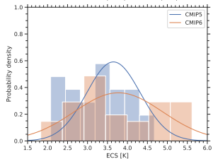
Sherwood et al. (2014) constraint (SHL)
