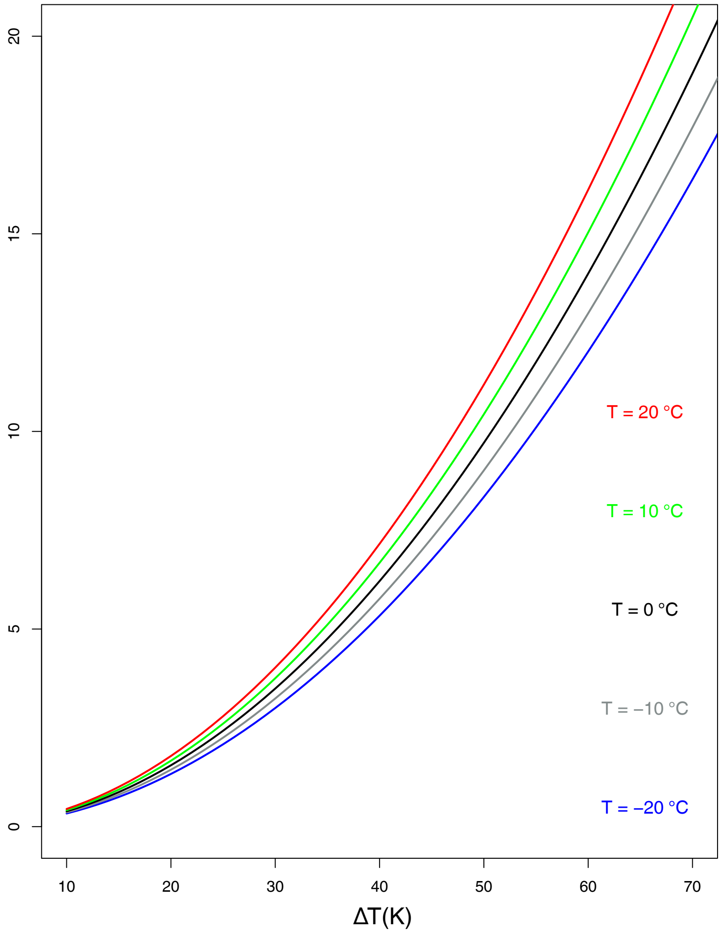
Change in longwave radiation ( \text{W m}^{-2} )
