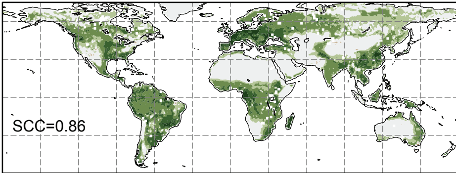
(b) Diff: SSIb4/TRIFFID minus GIMMS
