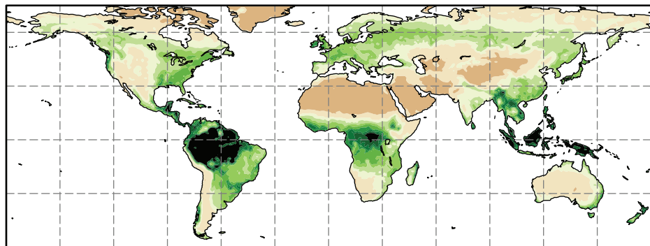
(c) GLASS LAI
