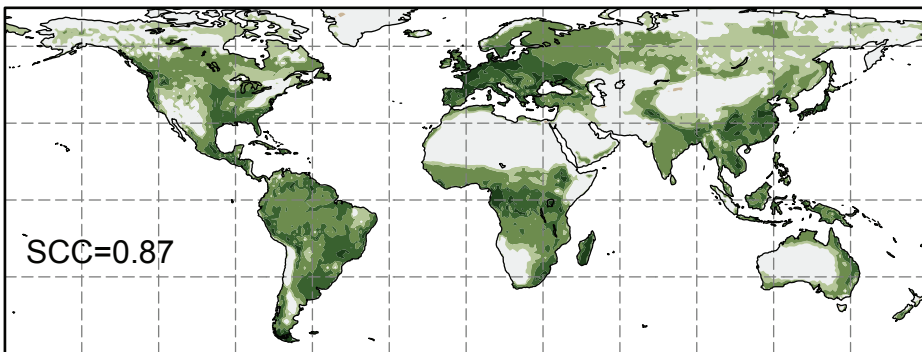
(d) Diff: SSIb4/TRIFFID minus GLASS
