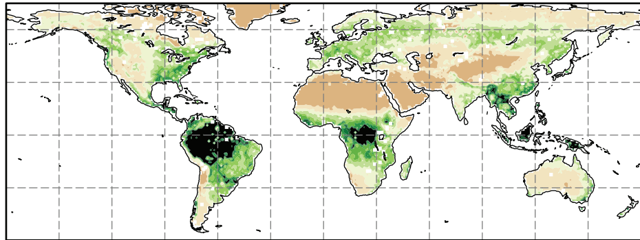
(a) GIMMS LAI
