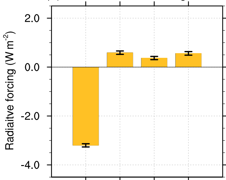
(b) TOA LW radiative forcing
