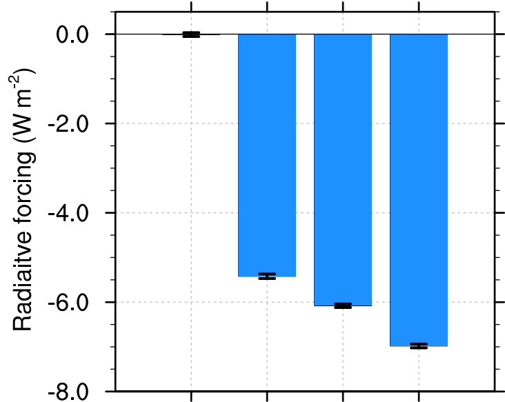
(e) TOA SWcld radiative forcing
