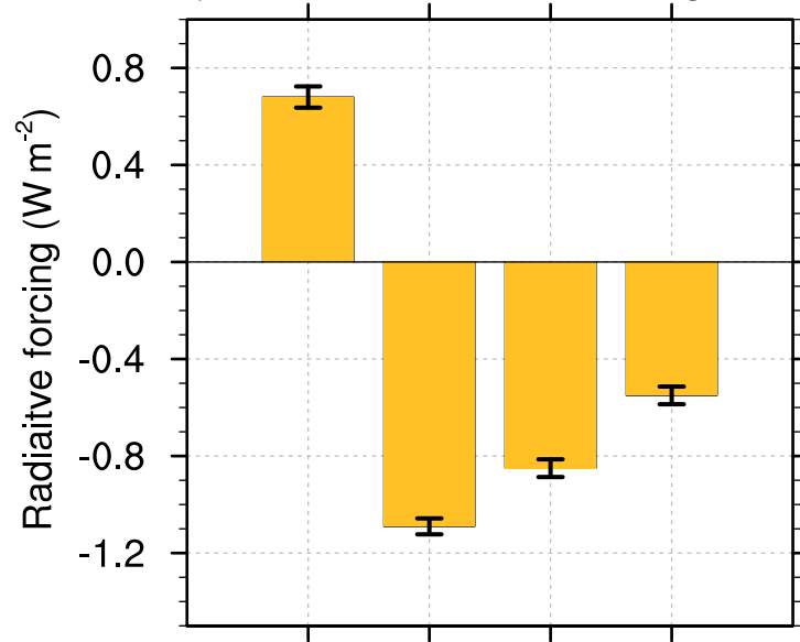
(f) TOA LWcld radiative forcing
