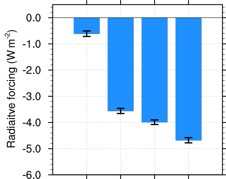
(a) TOA SW radiative forcing
