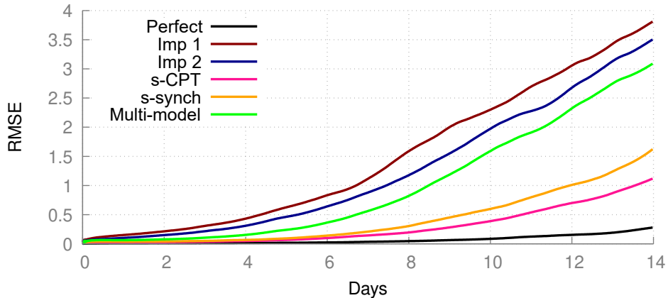
Temperature difference between model and truth
