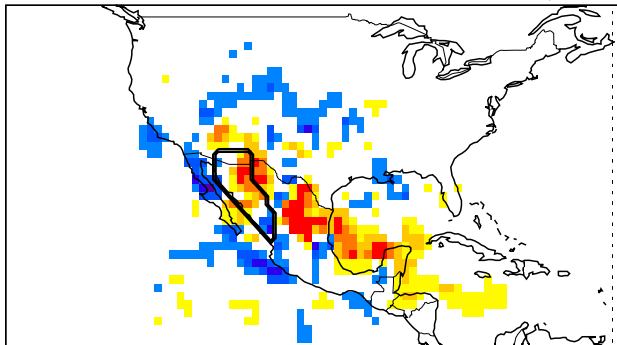
(c) E-P anom (ext-low) JA Day -5
