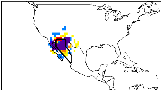
(a) E-P anom (ext-low) JA Day -1
