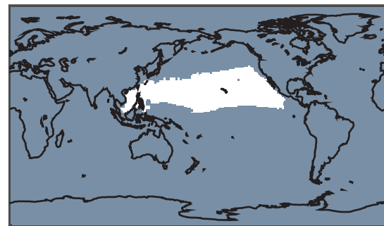
Biome 4: NP STPS
