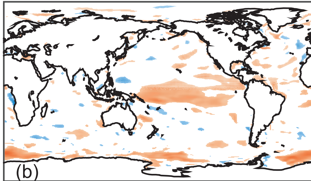
Uninitialized forecast
