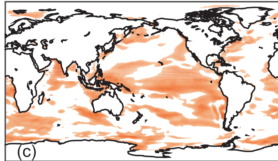
Persistence forecast
