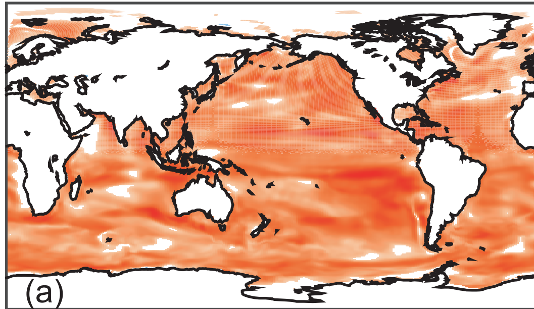
Initialized forecast
