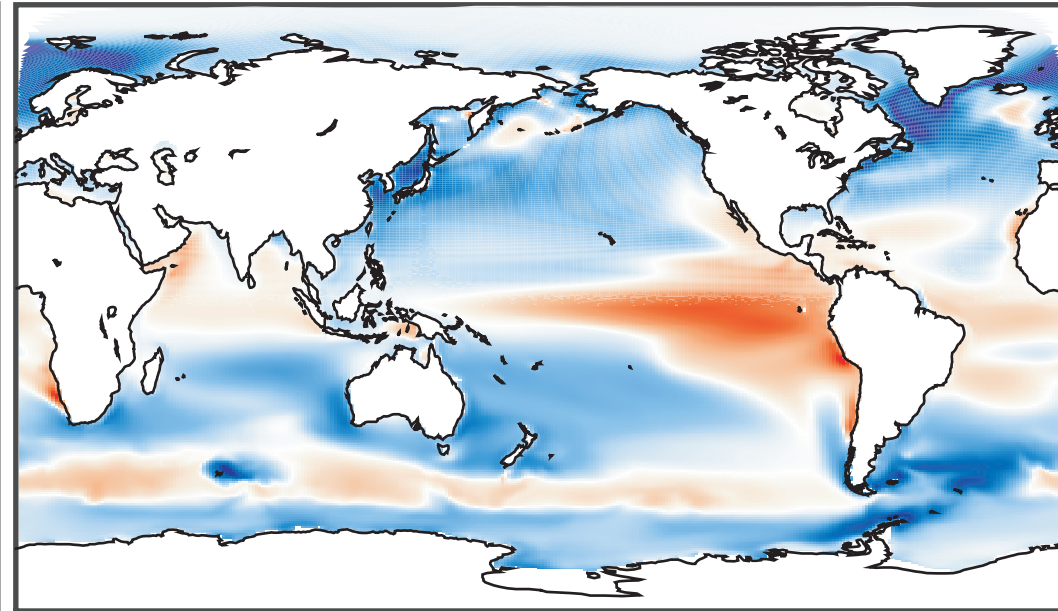
(c) CESM-LE
