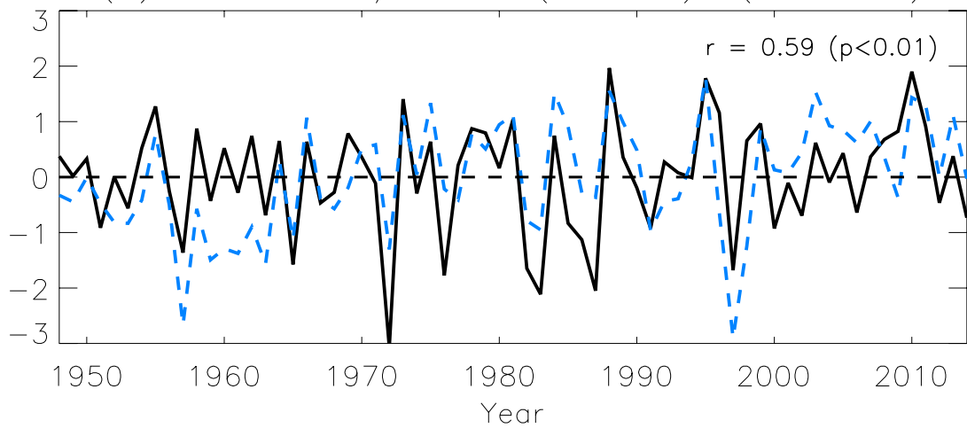
(b) \text{CHOCO-D} / \text{U925} (dashed) (Jun–Oct)
