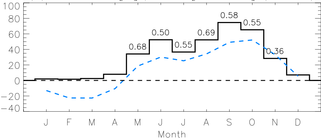
(a) \text{CHOCO-D} [\%] / \text{U925} [ * 10 \text{ m s}^{-1} ] (dashed)
