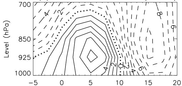
(c) Zonal wind at 90° W (m s -1 )
