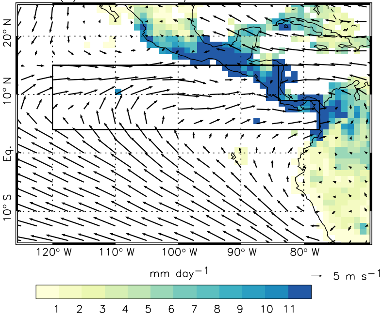
(a) GPCCv7+NCEP/NCAR 925 hPa wind
