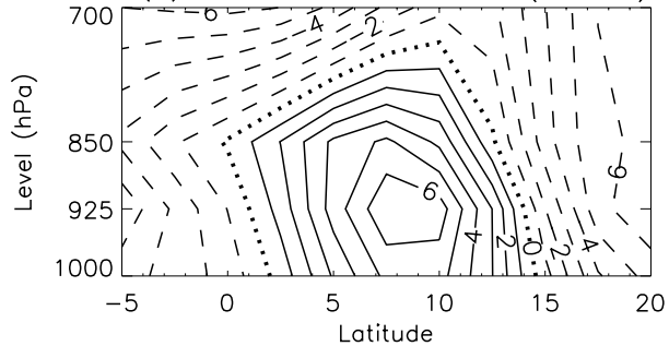
(c) Zonal wind at 90° W (m s -1 )
