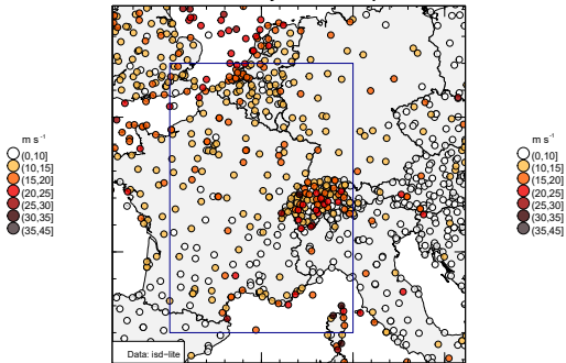
ELEANOR (2018-01-03) observed daily-max wind speed
