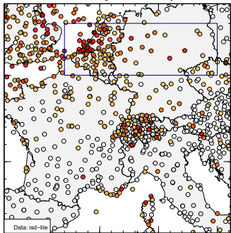
FRIEDERIEKE (2018-01-18) observed daily-max wind speed
