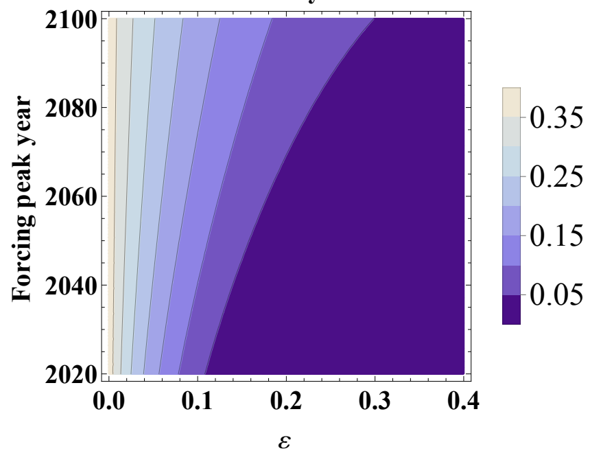
\tau=300 yr
