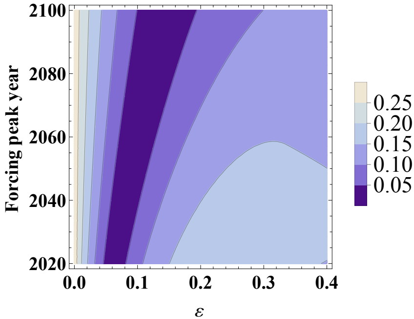
ECS=4K, \tau=300 yr
