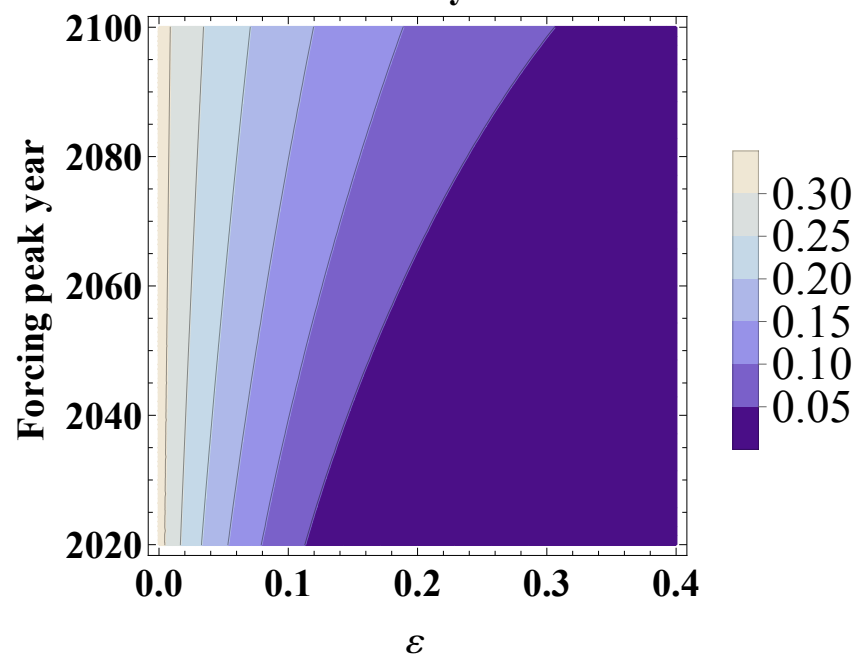
\tau=200 yr
