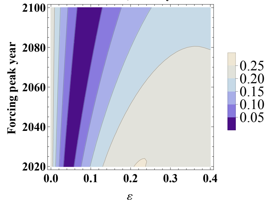
ECS=3K, \tau=300 yr
