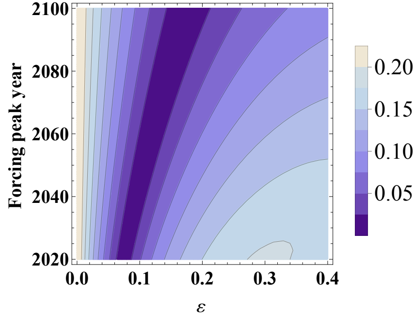
ECS=3K, \tau=200 yr
