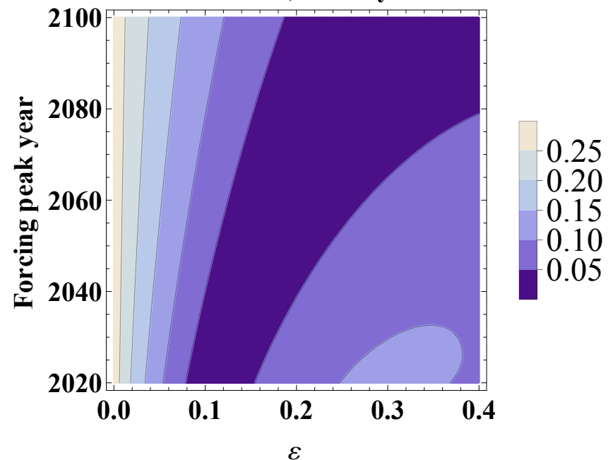
ECS=4K, \tau=200 yr
