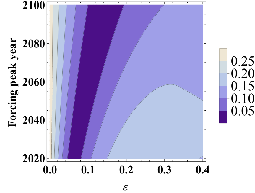
ECS=4K, \tau=300 yr
