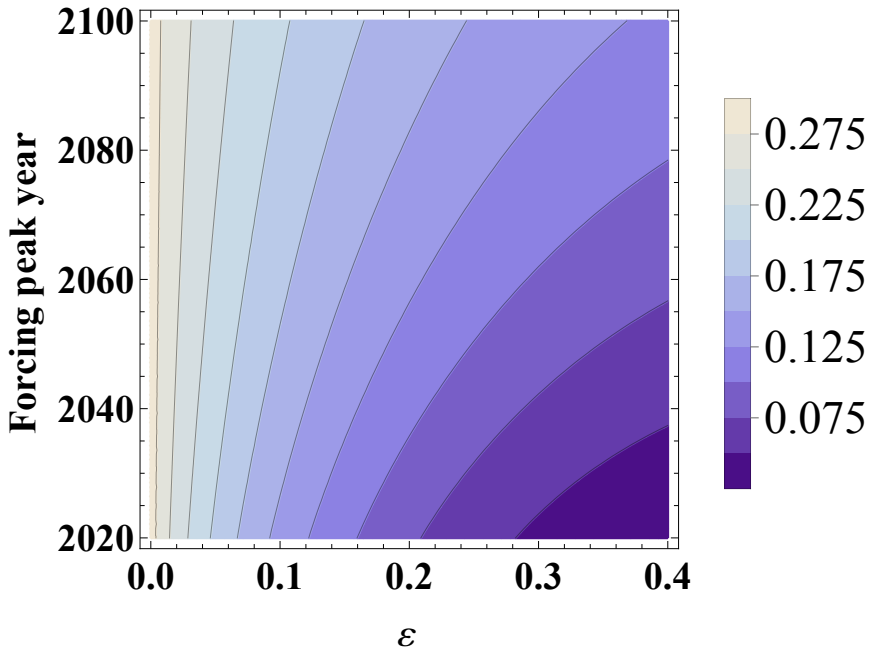
ECS=4K, \tau=100 yr
