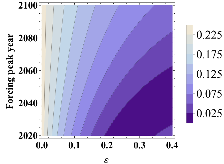
ECS=3K, \tau=100 yr
